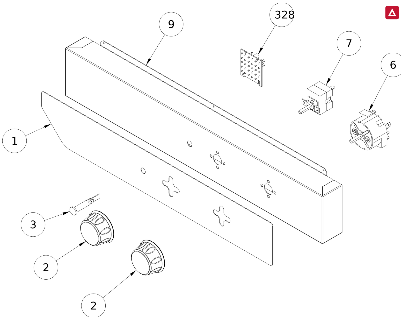
Frontal panel
